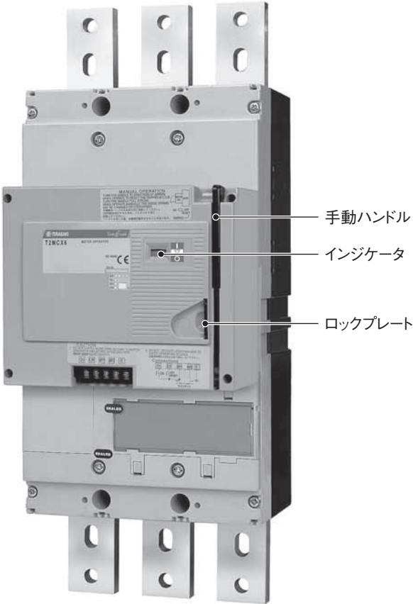
(T1MCX6形)
